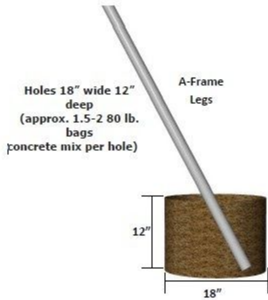
Hole Sizes for Cementing in the Set
